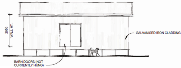
Front Elevation
